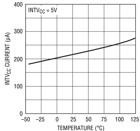
INTVCC Shutdown Current vs Temperature
